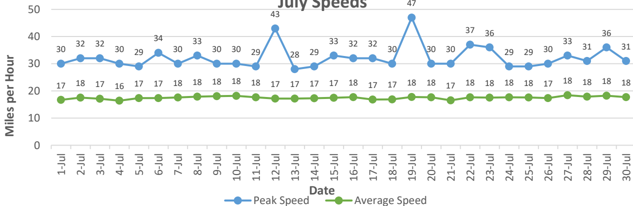
July Speeds
