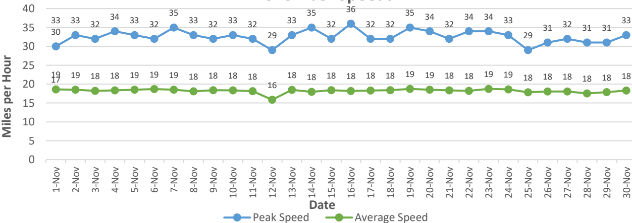
November Speeds
